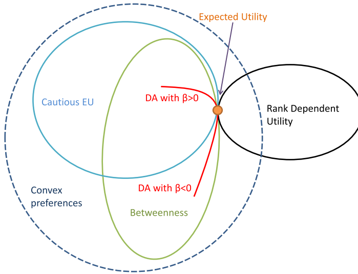
FIGURE 2.—Cautious expected utility and other models.
