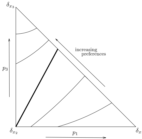
FIGURE 1.—NCI and the Marschak–Machina triangle.
